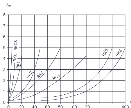
Figure 2: Q volumetric flow (lpm); Δp flow resistance (bar)
