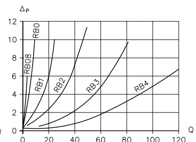
Figure 3: Q volumetric flow (lpm); Δp flow resistance (bar)
