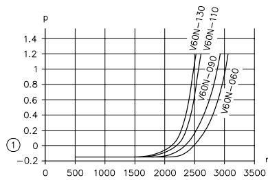
Figure 4: n rotation speed (rpm); p inlet pressure (bar)
