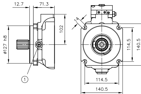
Coding F (SAE-C 4-hole) (127-4 ISO 3019-1)
