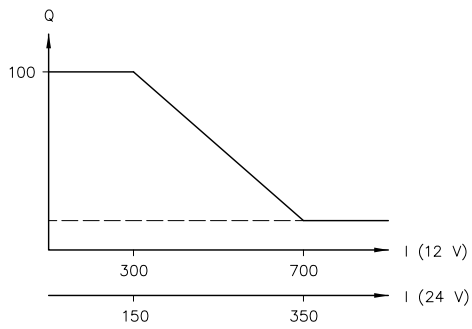
Figure 14: I current (mA); Q delivery flow (%)
