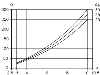
Figure 8: Ø orifice diameter (mm); Q delivery flow (%)
