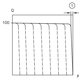
Figure 6: p B operating pressure (bar); Q delivery flow (%)
