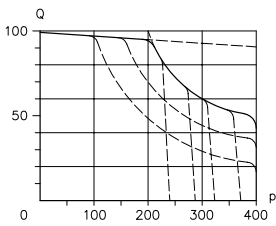
Figure 5: p pressure (bar); Q delivery flow (%)
