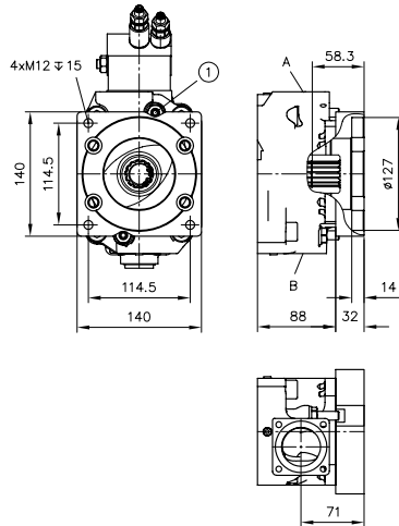
1 Stroke limitation
