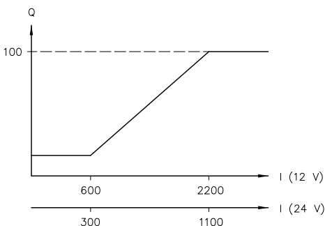
Figure 11: I current (mA); Q delivery flow (%)
