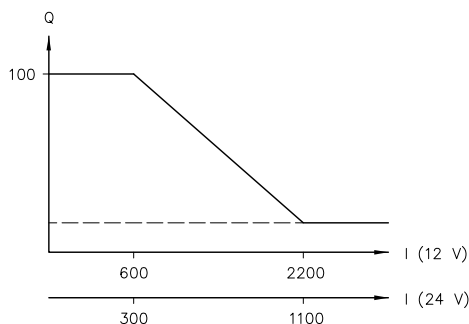
Figure 12: I current (mA); Q delivery flow (%)
