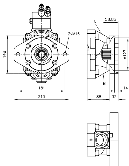
Coding C 027 (SAE-C 2-hole)
