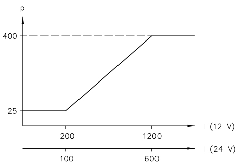
Figure 9: I current (mA); p pressure (bar)
