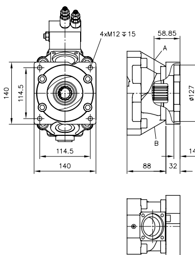
Coding C 028 (SAE-C 4-hole)
