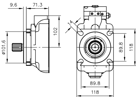
Coding Z (SAE-B 4-hole) (101-4 ISO 3019-1)
