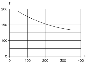
Figure 15: p pressure (bar); acting time T1 (ms)
