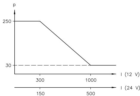
Figure 10: I current (mA); p pressure (bar)
