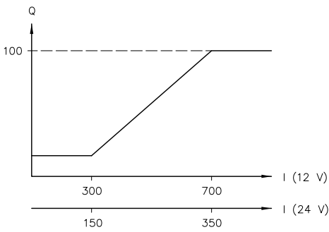
Figure 13: I current (mA); Q delivery flow (%)
